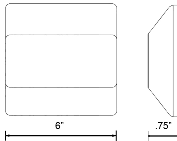
Type AI 6" Jiggle Bar White Ceramic Type AYI 6" Jiggle Bar Yellow Ceramic Packed 20 pieces per carton
